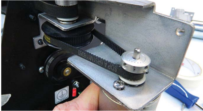
Step 9: The belt is around both the silver motor pulley as well as the black pulley.
