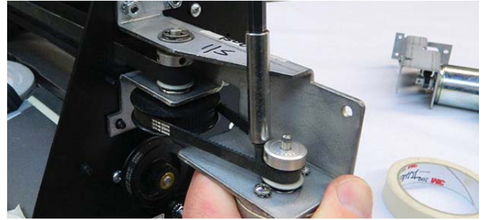
Step 10: Wrap your fingers around the motor and place your thumb at the end of the bracket as shown. Pull the motor tight (will see the belt tighten) and proceed to tighten all 3 screws.
