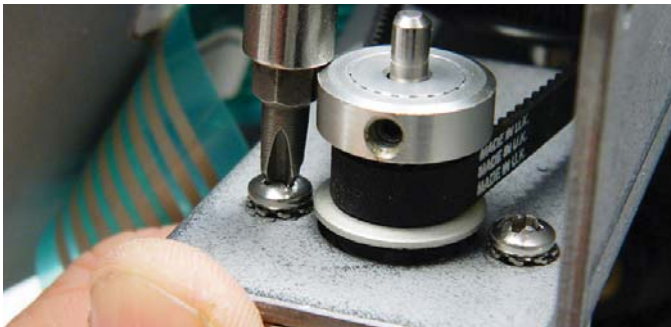
Step 11: Close up of a screw being tightened while tensioning the belt.
